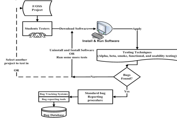
Figure 2. F/OSS Testing Strategy.
